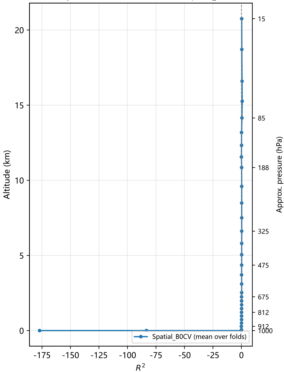
Per-layer R^2 of absolute extinction — Spatial_B0CV
