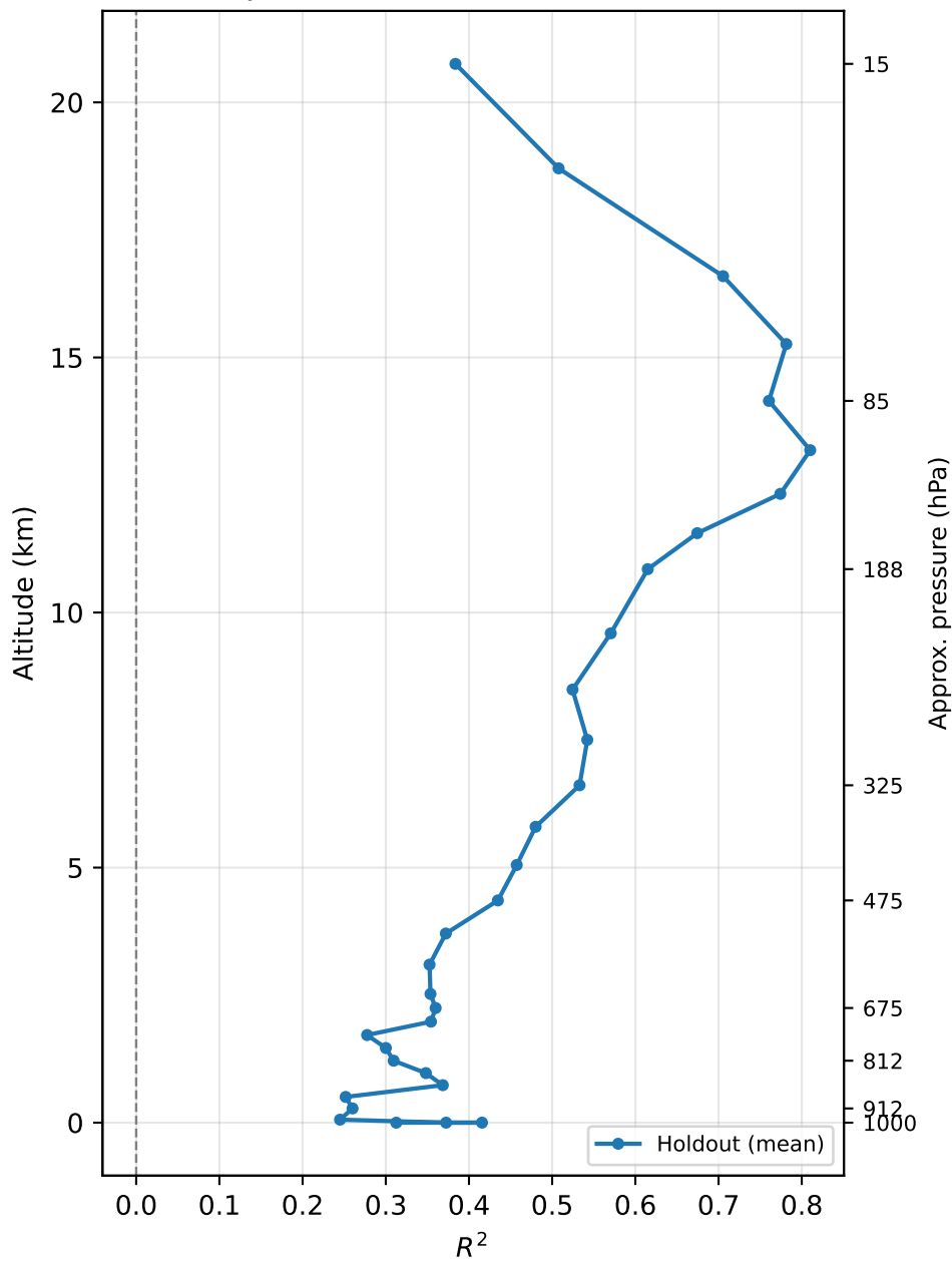
Per-layer R^2 of absolute extinction — Holdout
