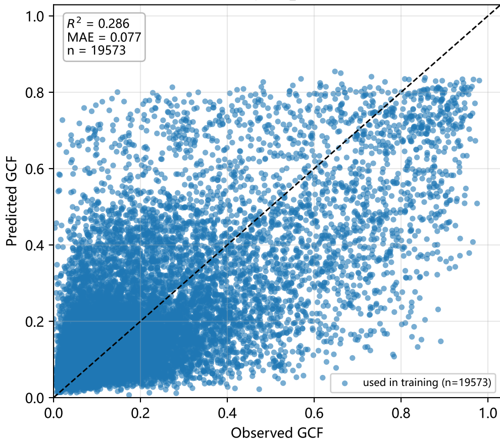
GCF — Spatial_AGLB0CV
