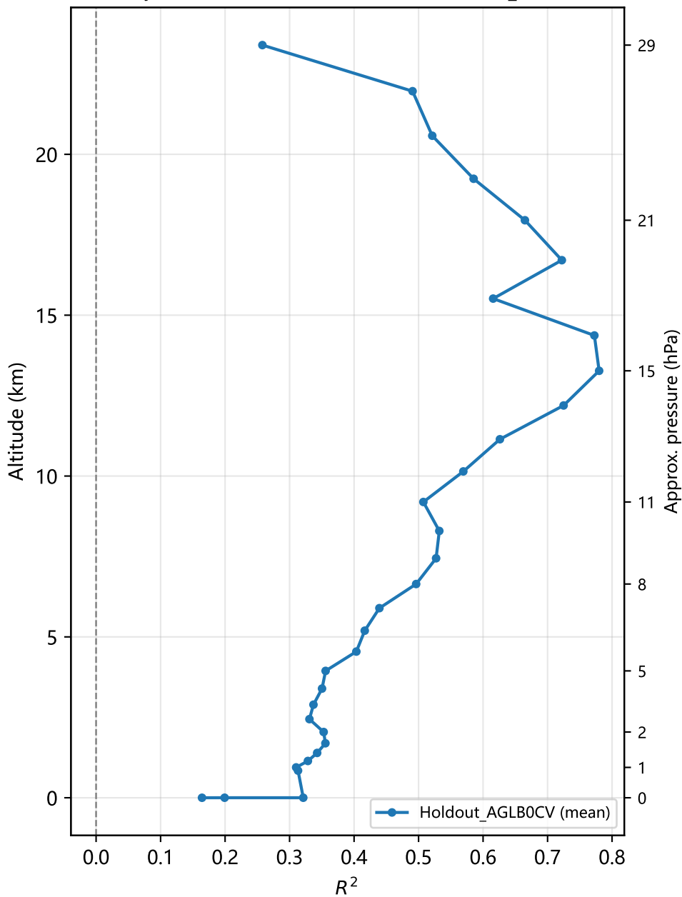
Per-layer R 2 of absolute extinction — Holdout_AGLB0CV
