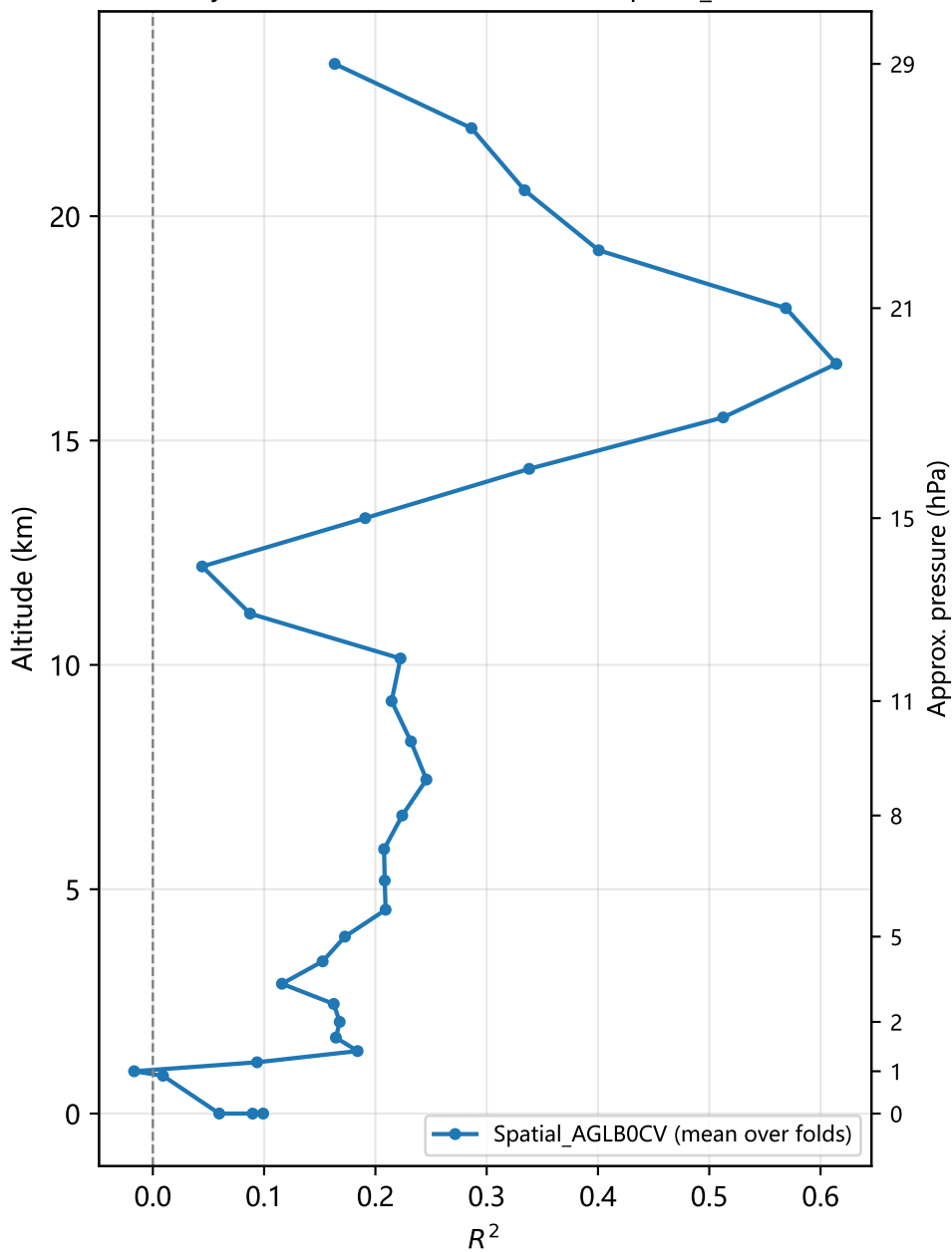
Per-layer R^2 of absolute extinction — Spatial_AGLB0CV
