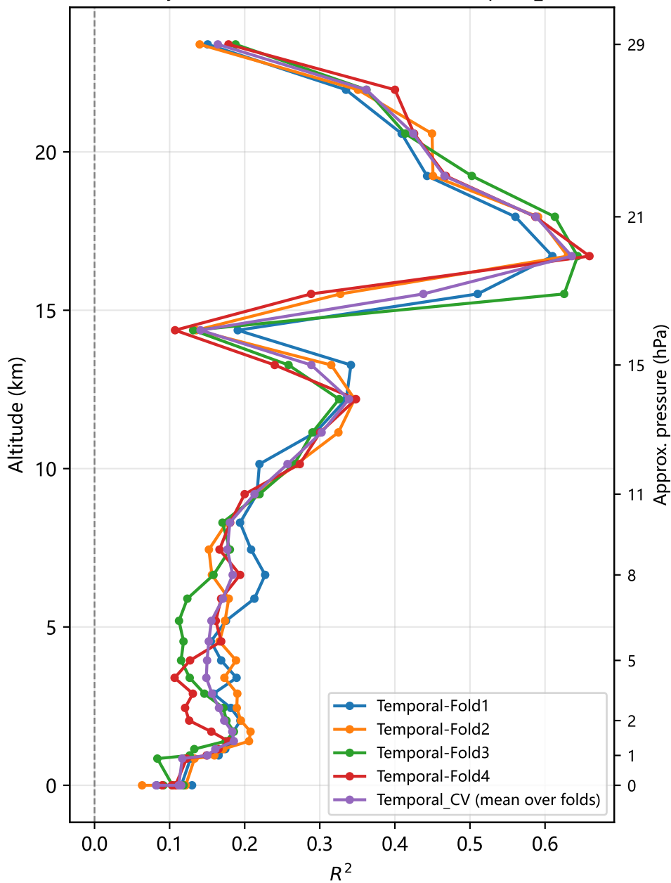
Per-layer R 2 of absolute extinction — Temporal_CV
