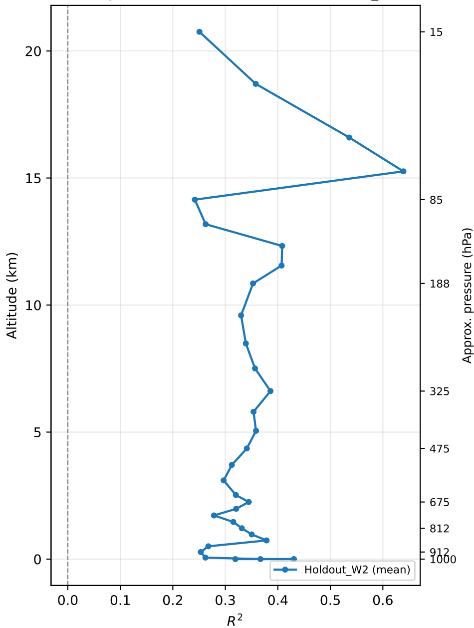
Per-layer R^2 of absolute extinction — Holdout_W2
