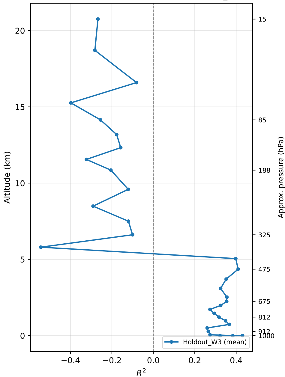
Per-layer R^2 of absolute extinction — Holdout_W3
