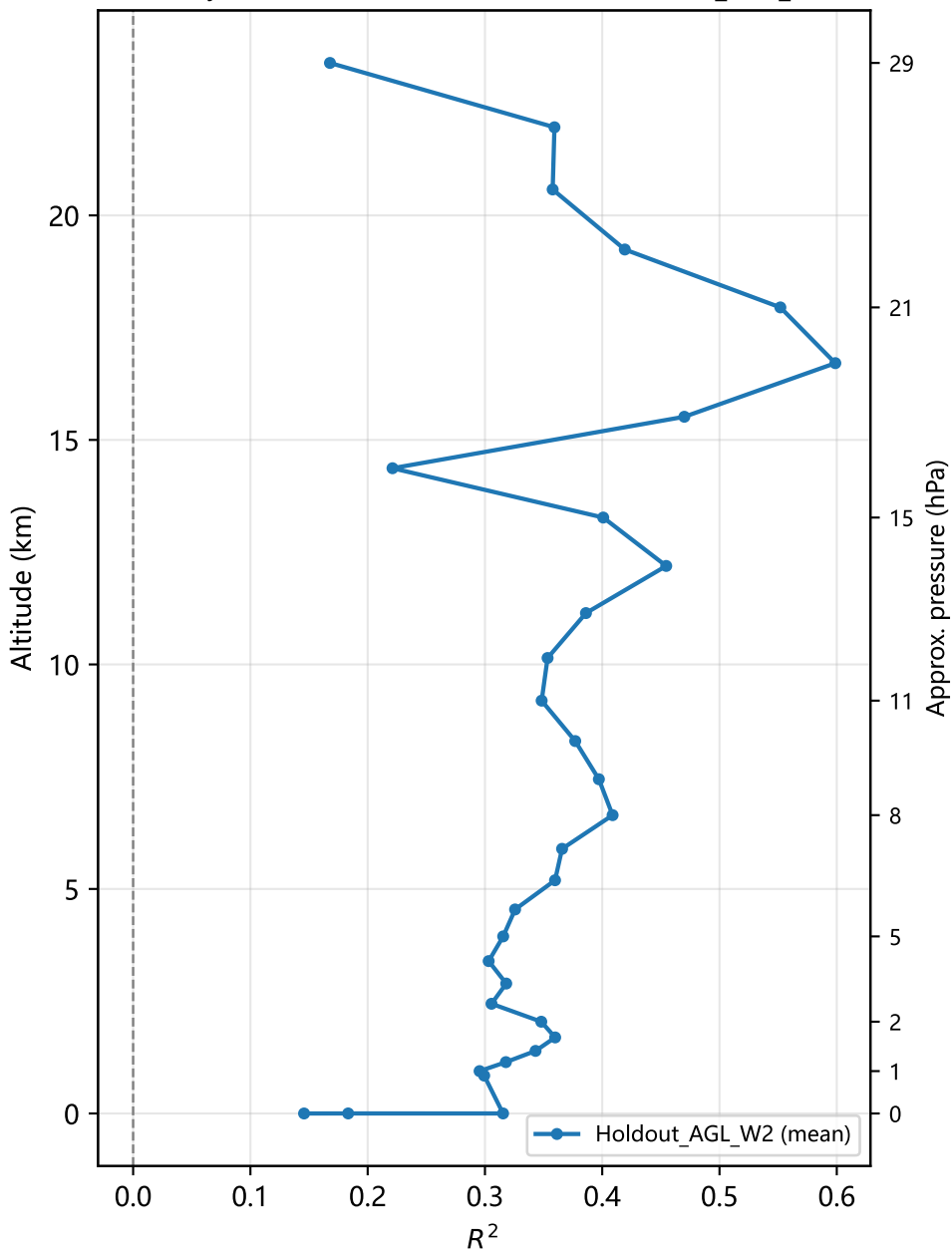
Per-layer R^2 of absolute extinction — Holdout AGL W2
