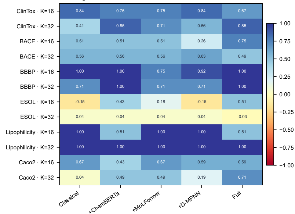
CAHit@3
