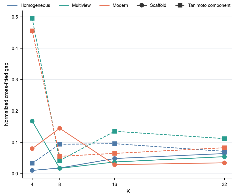
Composition effects across two evaluated split regimes
