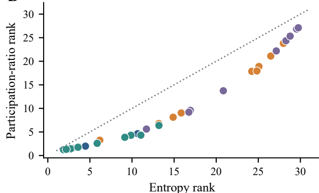
B Entropy and participation-ratio concordance
