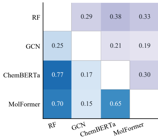
A Prediction and error similarity
