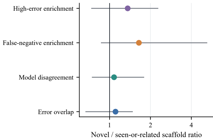
C Novel-scaffold reliability shifts
