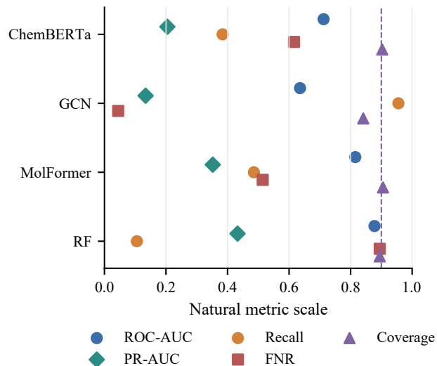
D ClinTox four-model trade-offs
