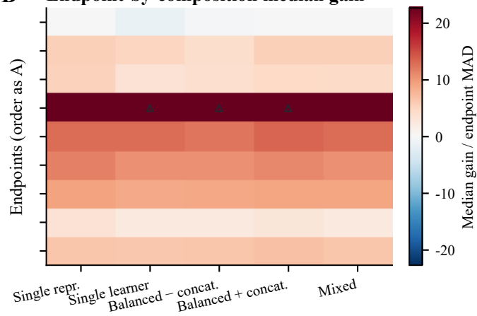
B Endpoint-by-composition median gain
