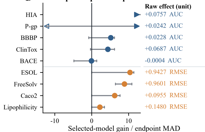
D Endpoint-specific representation effects
