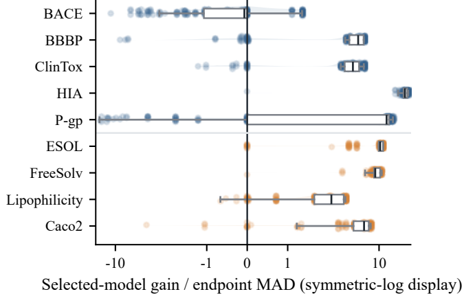
A Endpoint-specific K = 3 subset distributions
