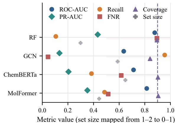
D ClinTox four-model trade-offs
