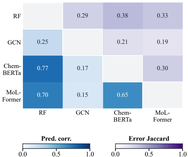
A Prediction and error similarity
