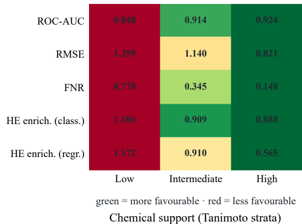
B Chemical-support performance and risk
