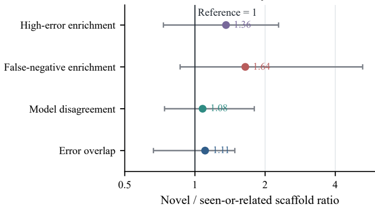
C Novel-scaffold reliability shifts
