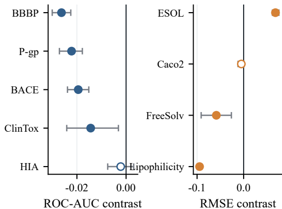
C K-invariant full-registry effects
