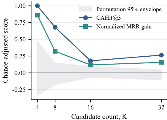
A Chance-adjusted top-rank recovery
