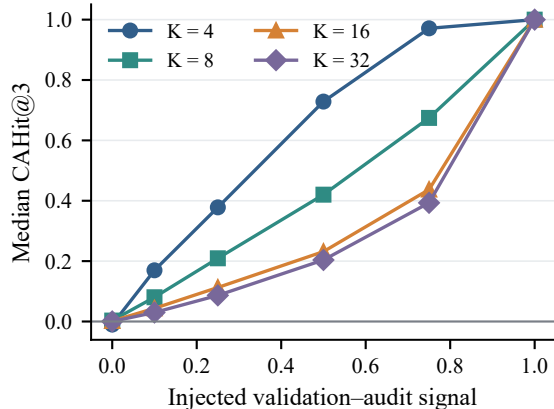
B Signal-recovery calibration
