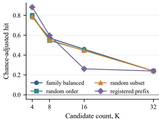
D Candidate-composition controls
