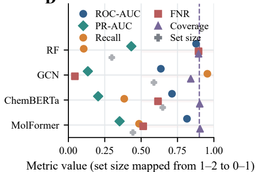
D ClinTox four-model trade-offs
