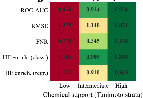
B Chemical-support performance and risk
