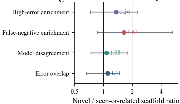
C Novel-scaffold reliability shifts
