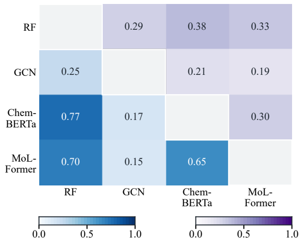
A Prediction and error similarity
