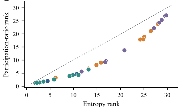
B Entropy and participation-ratio concordance
