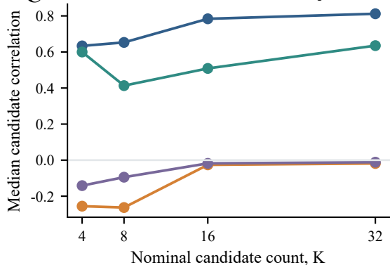
C Candidate correlation after adjustment
