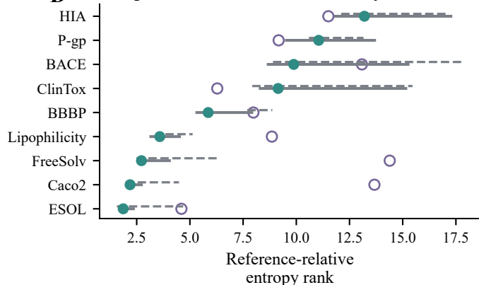
D Endpoint and reference sensitivity
