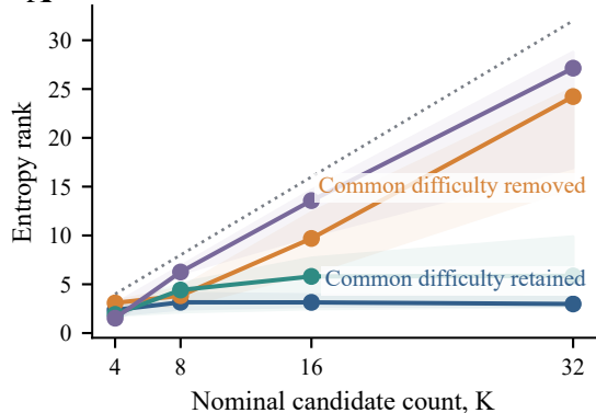
A Effective diversity across K
