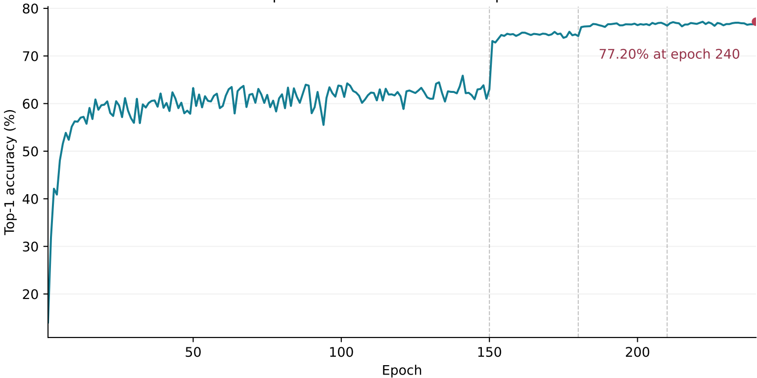
CIFAR-100 | ResNet32x4 to ResNet8x4 | UATM + UGSA
