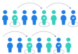
系统采样 (Systematic Sampling)
