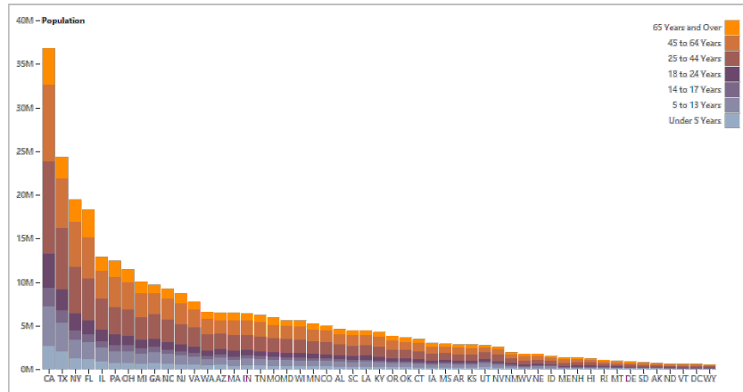
Stacked Bar Chart
