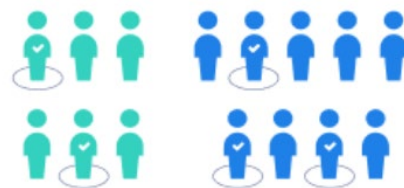
分层采样 (Stratified Sampling)
