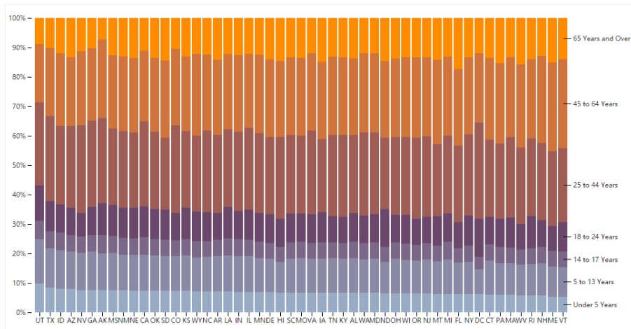
Normalized Stacked Bar Chart
