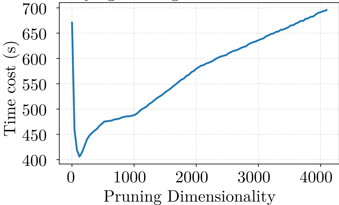
Varying Pruning Dims on HDR-Tree
