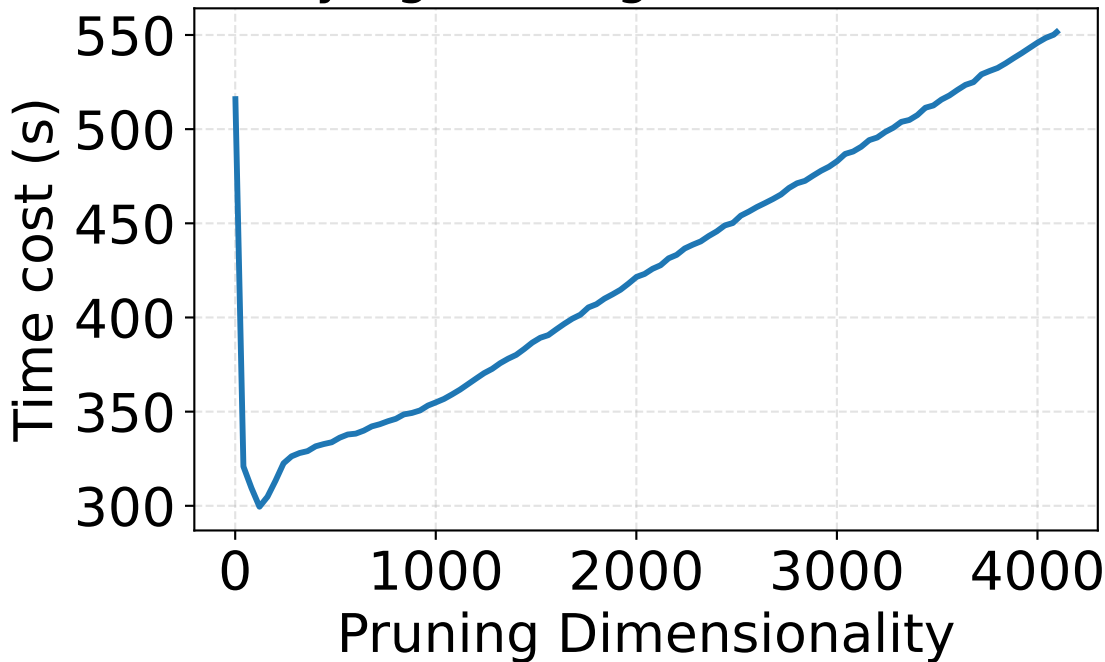
Varying Pruning Dims on \Delta -Tree
