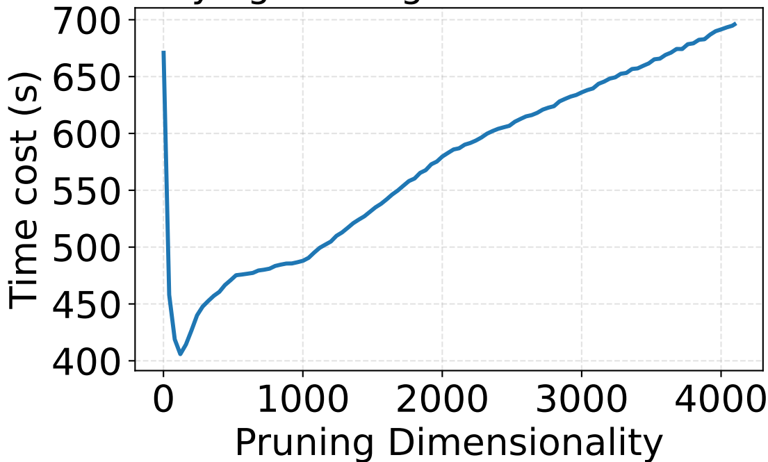
Varying Pruning Dims on HDR-Tree
