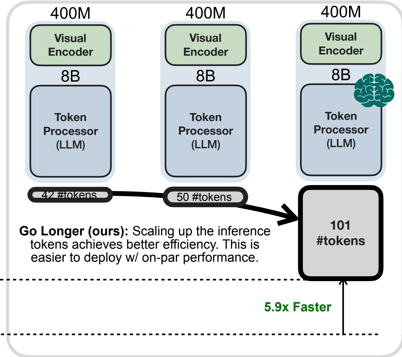
(b). Our EGM scales test-time-inference .
