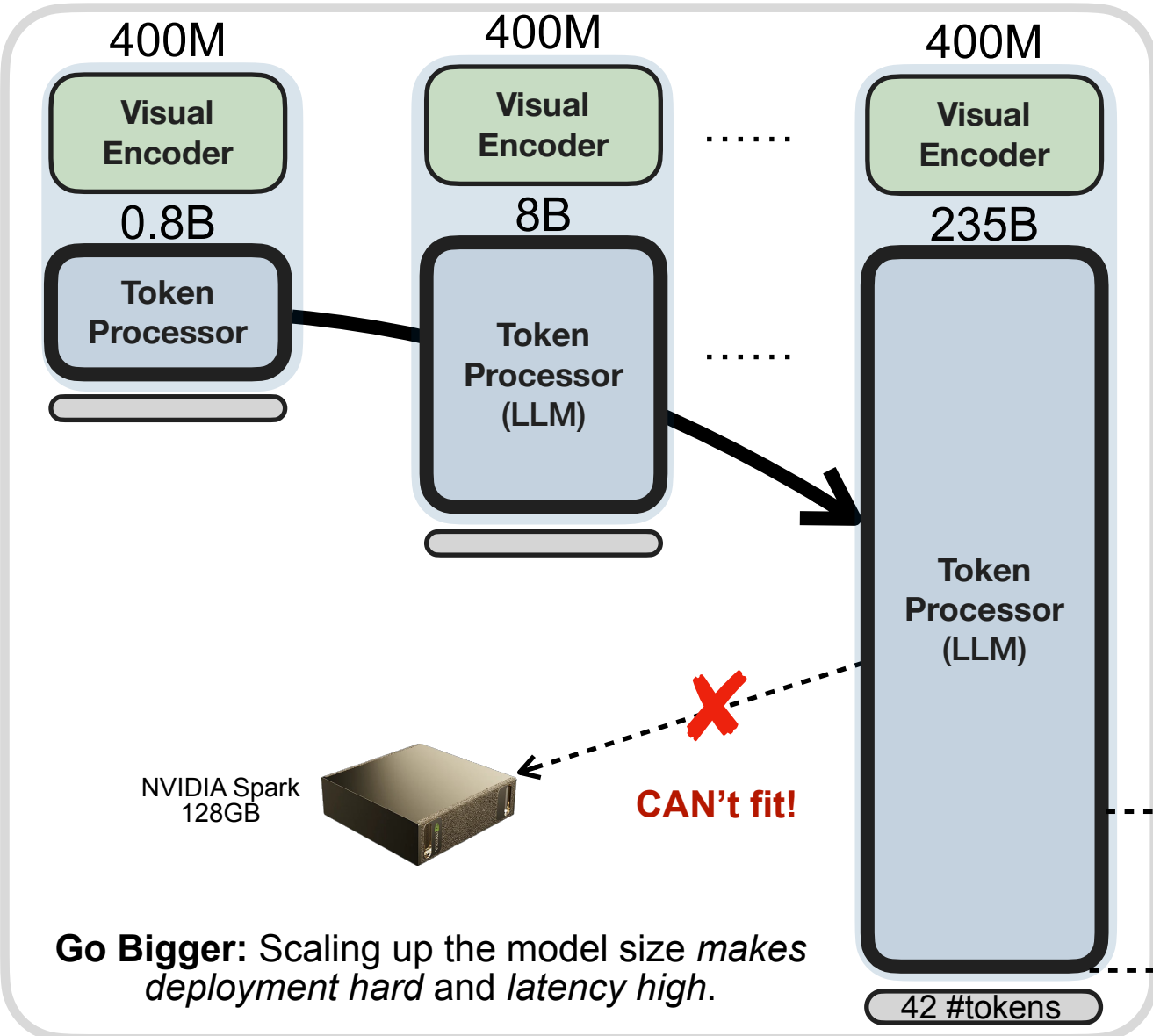
(a). Conventional grounding VLMs scale the size of LLM
