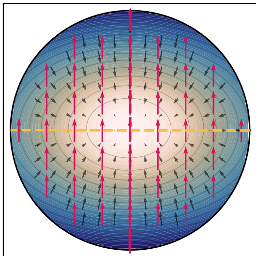
intrinsic (transport)
