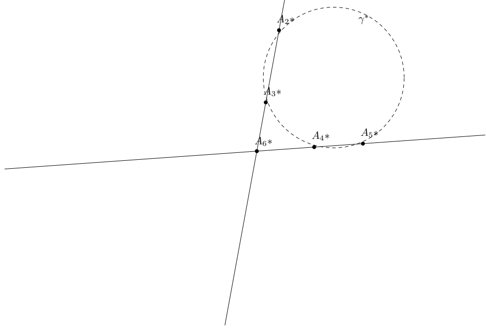
Figure 7: A_6^* is the intersection of lines A_2^*A_3^* and A_4^*A_5^* .
