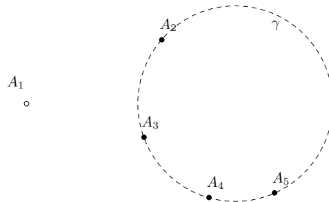
Figure 6: A_2A_3A_4A_5 lie on a circle \gamma not containing A_1 .
