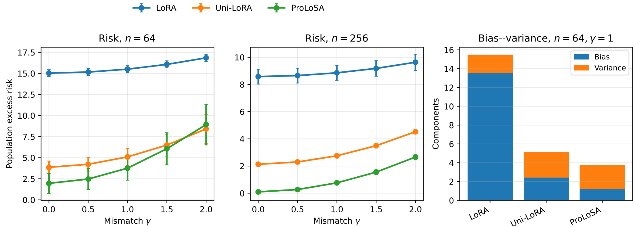
Figure S1: Known-projection synthetic validation of the bias-variance theory. Left and middle: population excess risk as subspace mismatch \gamma increases under different sample sizes. Right: empirical bias-variance decomposition at n=64 and \gamma=1 . ProLoSA uses warmup SNIP scores to select sparse residual coordinates.
