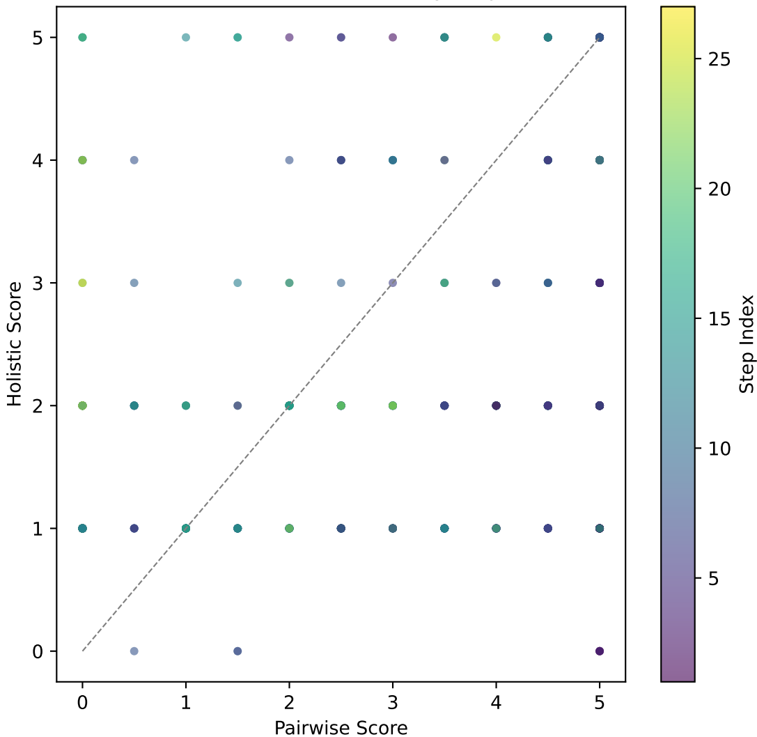
Pairwise vs Holistic (colored by step index)
