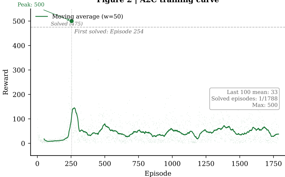
Figure 2 | A2C training curve
