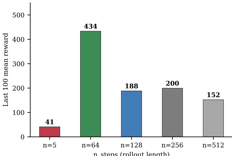
A2C n_steps effect
