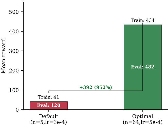
Figure S3 | Default vs optimal A2C
