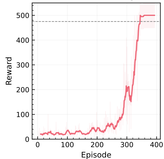
(a) PPO Training
