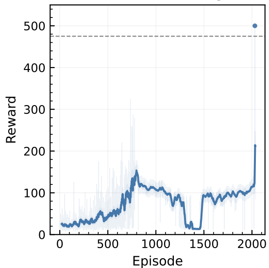
(b) DQN Training
