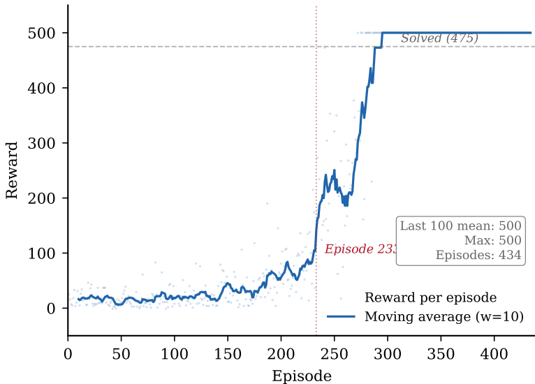
Figure 1 | PPO training curve
