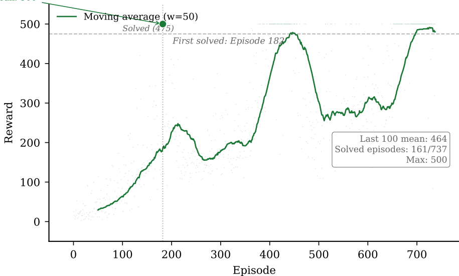
Figure 2 | A2C training curve
