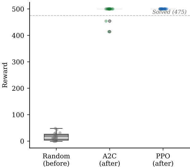
Figure 5 | Before vs after training
