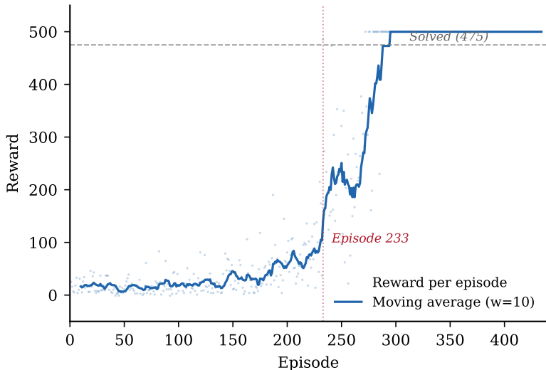
Figure 1 | PPO training curve
