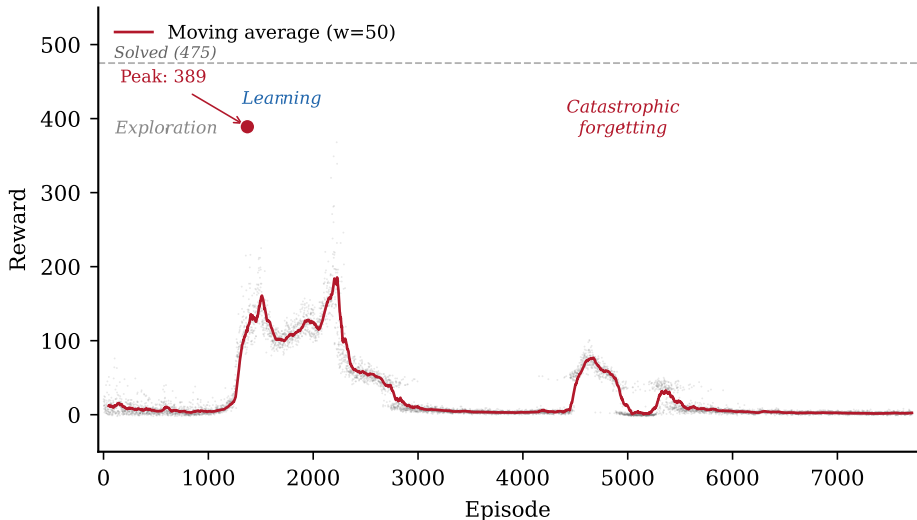
Figure 2 | DQN training curve — catastrophic forgetting
