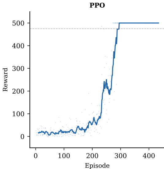
Figure 4 | Training process comparison
