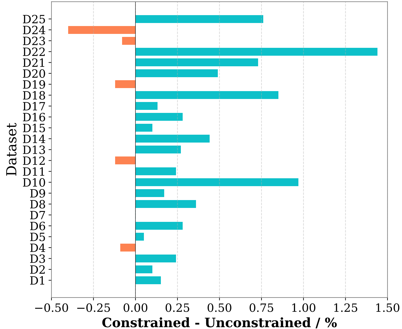
F1-Score
