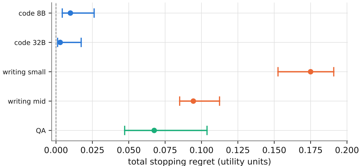
Total regret remains largest in critic-driven writing
