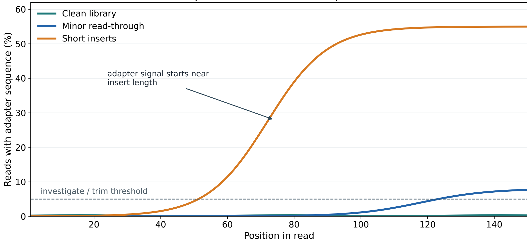
Adapter content across read positions
