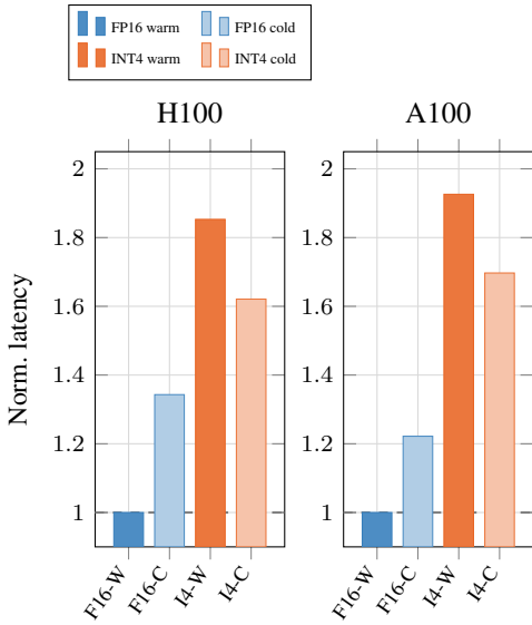
Figure 4: Cache-residency intervention at fixed MLA reconstruction shape (BS=1, normalized to FP16-warm). H100: eviction adds +4.8 \mu s to FP16 (= full 16 MB weight reload at HBM rate) and +3.9 \mu s to INT4, of which \sim 2.6 \mu s is common-mode eviction overhead (expected INT4 reload: 1.3 \mu s). The FP16 delta supports L2-residency dependence of the FP16 path; note that absolute deltas, not relative percentages, are the comparable quantity here since the two baselines differ \sim 2.6\times .
