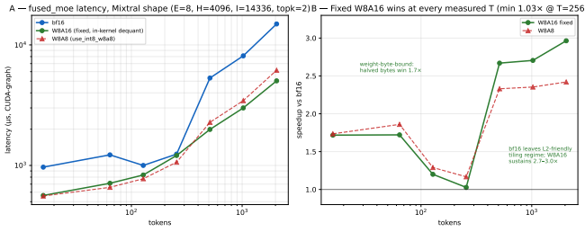
Figure 11: FlagGems fused_moe, Mixtral shape, graph-timed ( T=16 –2048). A : latency for bf16, fixed W8A16 (in-kernel dequant), and W8A8. B : speedup over bf16 — the fixed W8A16 kernel wins at every measured token count, 2.7 – 3.0\times at T\geq 512 .
