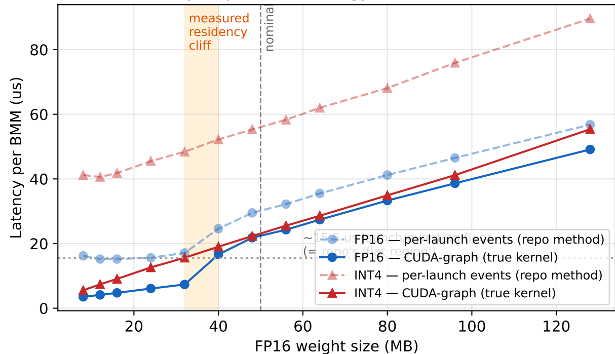
Latency: repo methodology vs true kernel time
