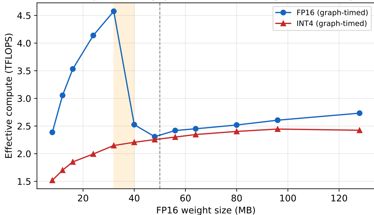
Useful FLOP throughput: max ~4.6 TFLOPS = 0.5% of peak (989 TF) neither kernel is compute-throughput bound; INT4's high SM% is dequant overhead
