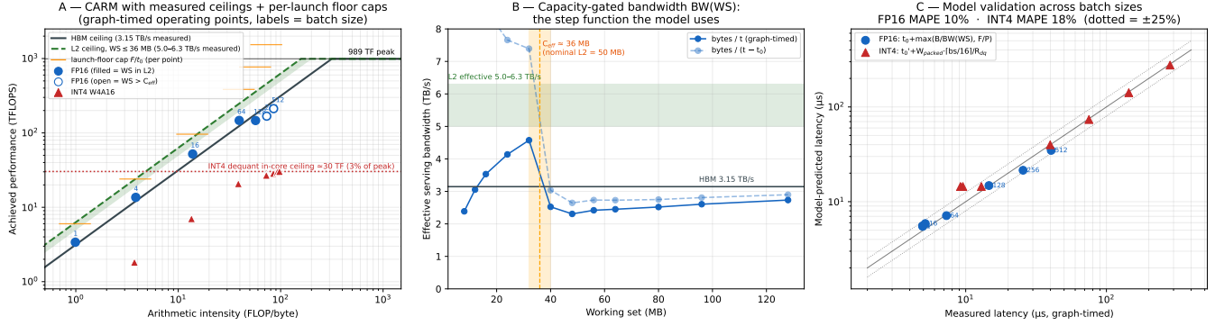
Figure 11: Measured cache-aware roofline for MLA reconstruction (H100, graph-timed). A: CARM with measured HBM and L2 ceilings, per-point launch-floor caps, and the fitted INT4 dequant in-core ceiling ( \sim 30 TF); FP16 points (labeled by batch size) are filled when the working set fits C_{eff} . B: the capacity-gated bandwidth function BW(WS) — effective serving bandwidth vs. working set, with the measured residency cliff at 32–40 MB. C: model validation, predicted vs. measured latency (dotted = \pm 25\% ).
