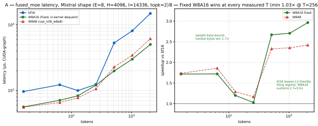
Figure 14: FlagGems fused_moe, Mixtral shape, graph-timed (T=16–2048). A : latency for bf16, fixed W8A16 (in-kernel dequant), and W8A8. B : speedup over bf16 — the fixed W8A16 kernel wins at every measured token count, 2.7–3.0 \times at T \geq 512.
