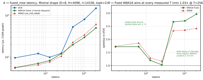
Figure 11: FlagGems fused_moe, Mixtral shape, graph-timed (T=16–2048). A : latency for bf16, fixed W8A16 (in-kernel dequant), and W8A8. B : speedup over bf16 — the fixed W8A16 kernel wins at every measured token count, 2.7–3.0× at T \geq 512 .
