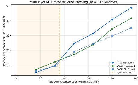
Figure 10: Multi-layer MLA reconstruction stacking (bs=1, 16 MB/layer, graph-timed). Stacking 1–6 layers sweeps the per-step working set from 16 to 96 MB; the FP16→W8A8 crossover occurs between two and three layers (32→48 MB), bracketing the measured C_{\text{eff}} \approx 36 MB. Dashed: CARM FP16 prediction.
