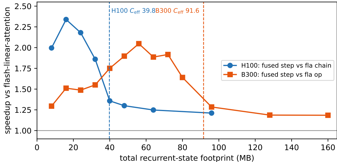
Residency-aware GDN decode: the speedup window tracks measured C_{\text{eff}}
