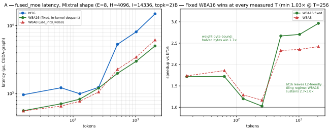
Figure 11: FlagGems fused_moe, Mixtral shape, graph-timed (T=16–2048). A: latency for bf16, fixed W8A16 (in-kernel dequant), and W8A8. B: speedup over bf16 — the fixed W8A16 kernel wins at every measured token count, 2.7–3.0× at T≥512.
