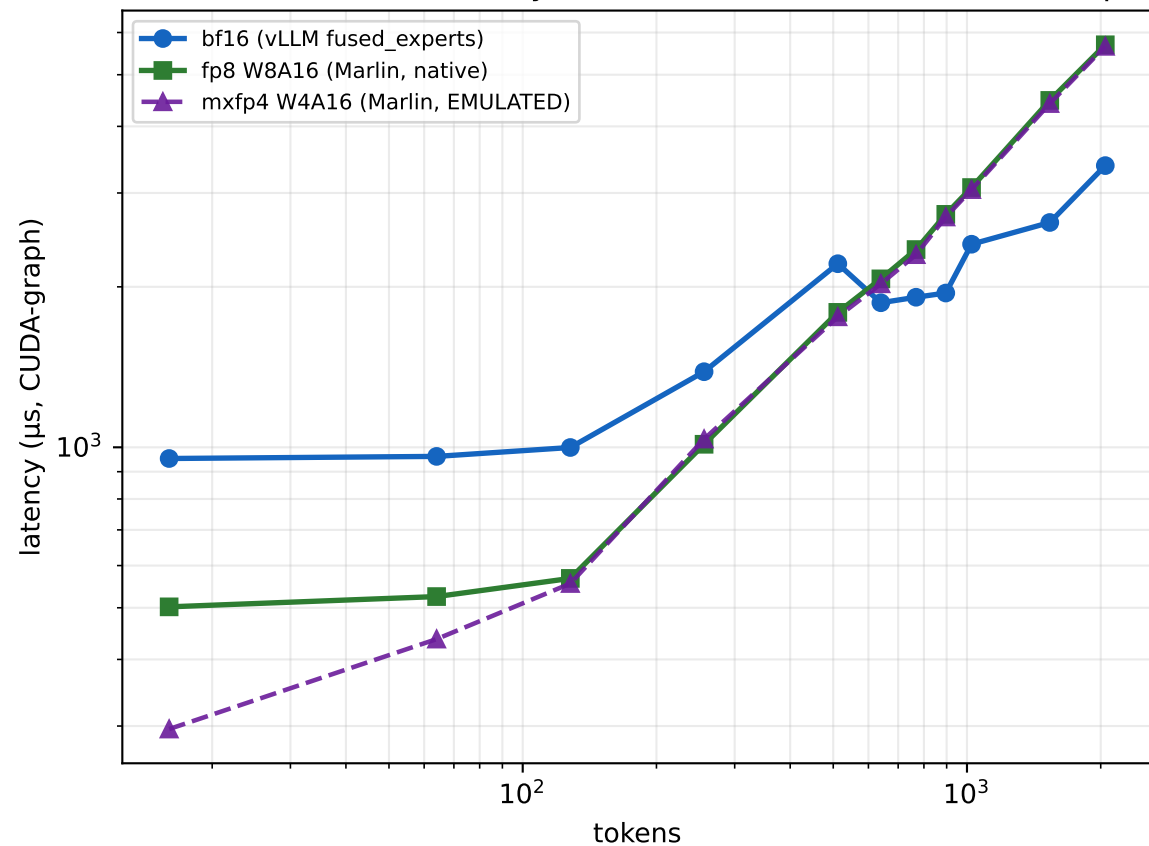
A — tuned-CUDA MoE latency (Mixtral E=8,H=4096,l=14336,topk=2)
