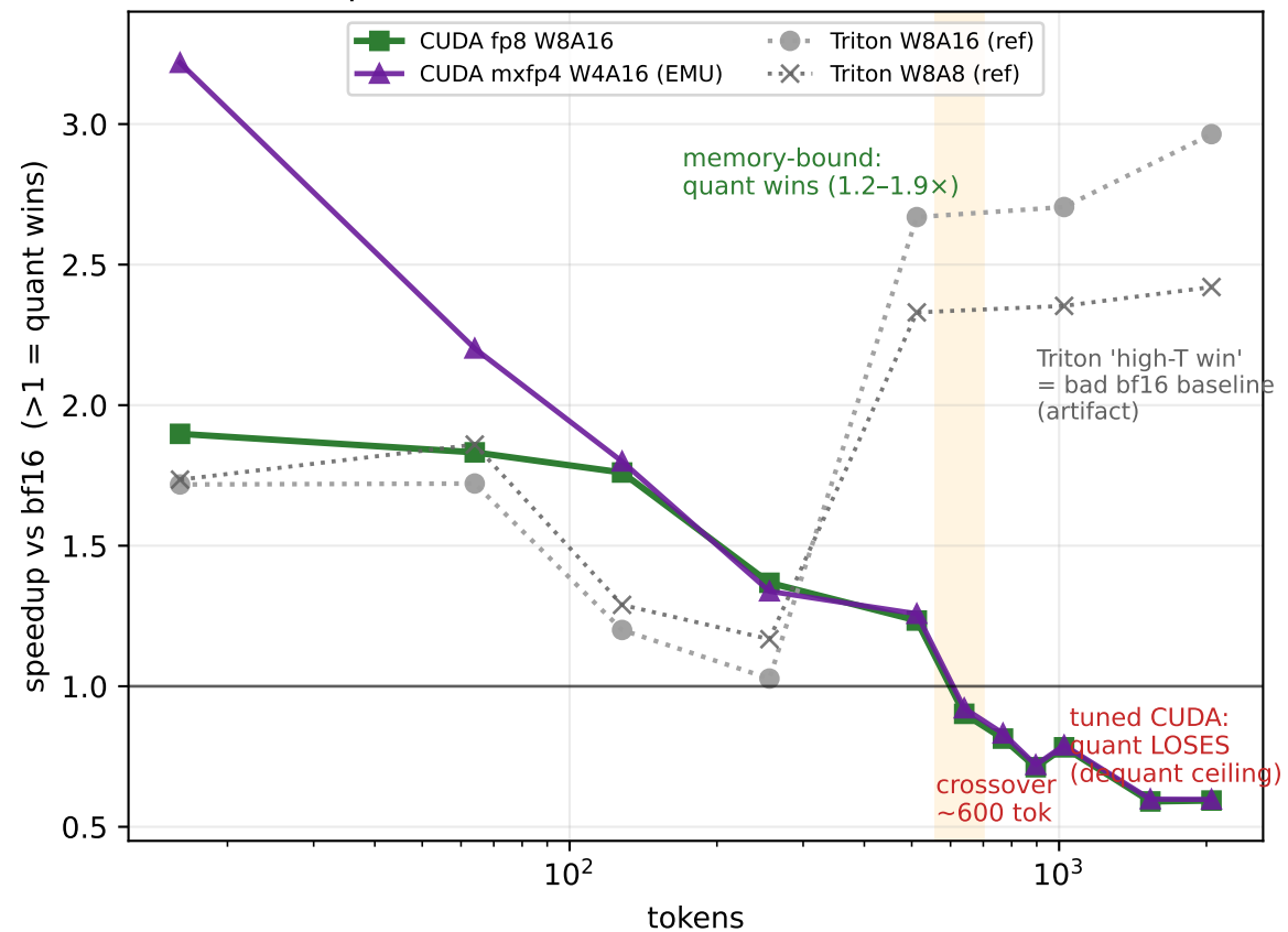
B — CUDA quant crosses below 1.0 at ~600 tok; Triton did not
