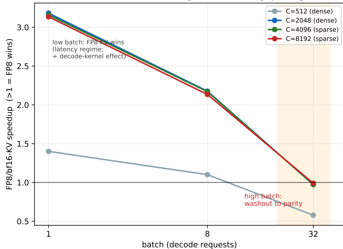
B — FP8 KV washes out at high batch (throughput regime)
