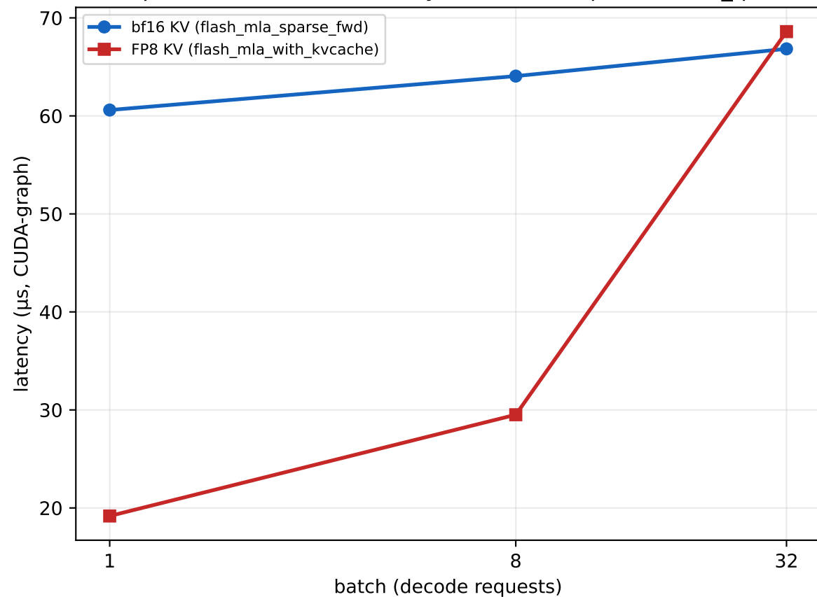
A — sparse MLA decode latency (C=4096, topk=2048, h_q=128)
